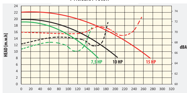
Pritisak/Protok
