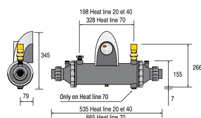
Heat Line Plus bez cirkulacione pumpe
