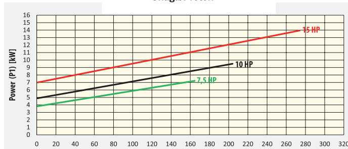
Snaga/Protok
